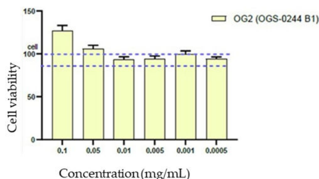
Figure 5. Evaluation of cytotoxicity of OG2 polyphenolic extract on HEKa cells.
